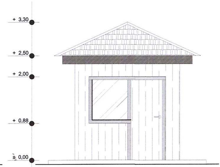
TAMPAK SAMPING KIRI BOOTH SKALA 1 : 50
