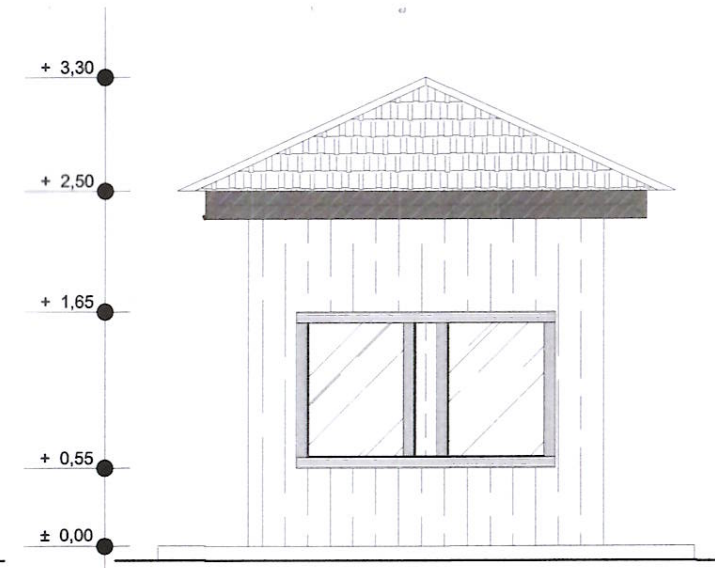
TAMPAK SAMPING KANAN BOOTH SKALA 1 : 50
